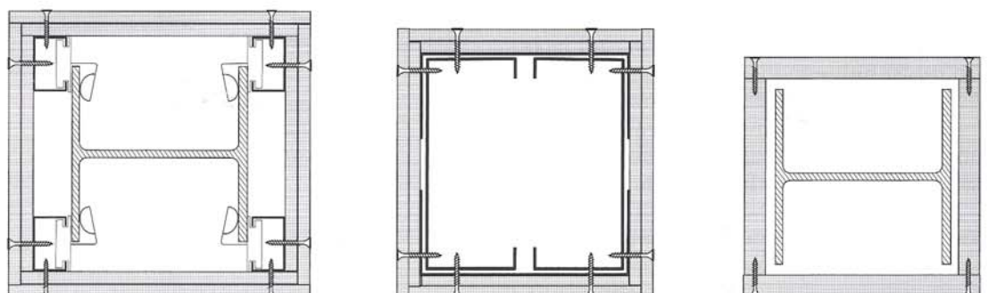
Fig. 114: Facing of steel sections with gypsum material plates for fire protection
