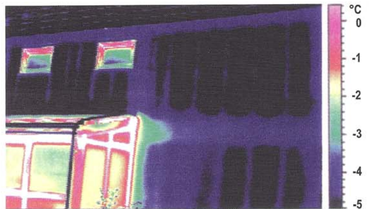
Fig. 83, 84 (below): Web of a "thermal profile" and heat flux through the cross section
