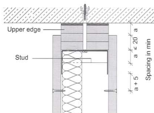
Fig. 107: Sliding ceiling junction of a nonstructural wall with fire protection requirements
